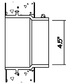
RUBBER BOOT DETAIL
