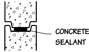
JOINT DETAIL
